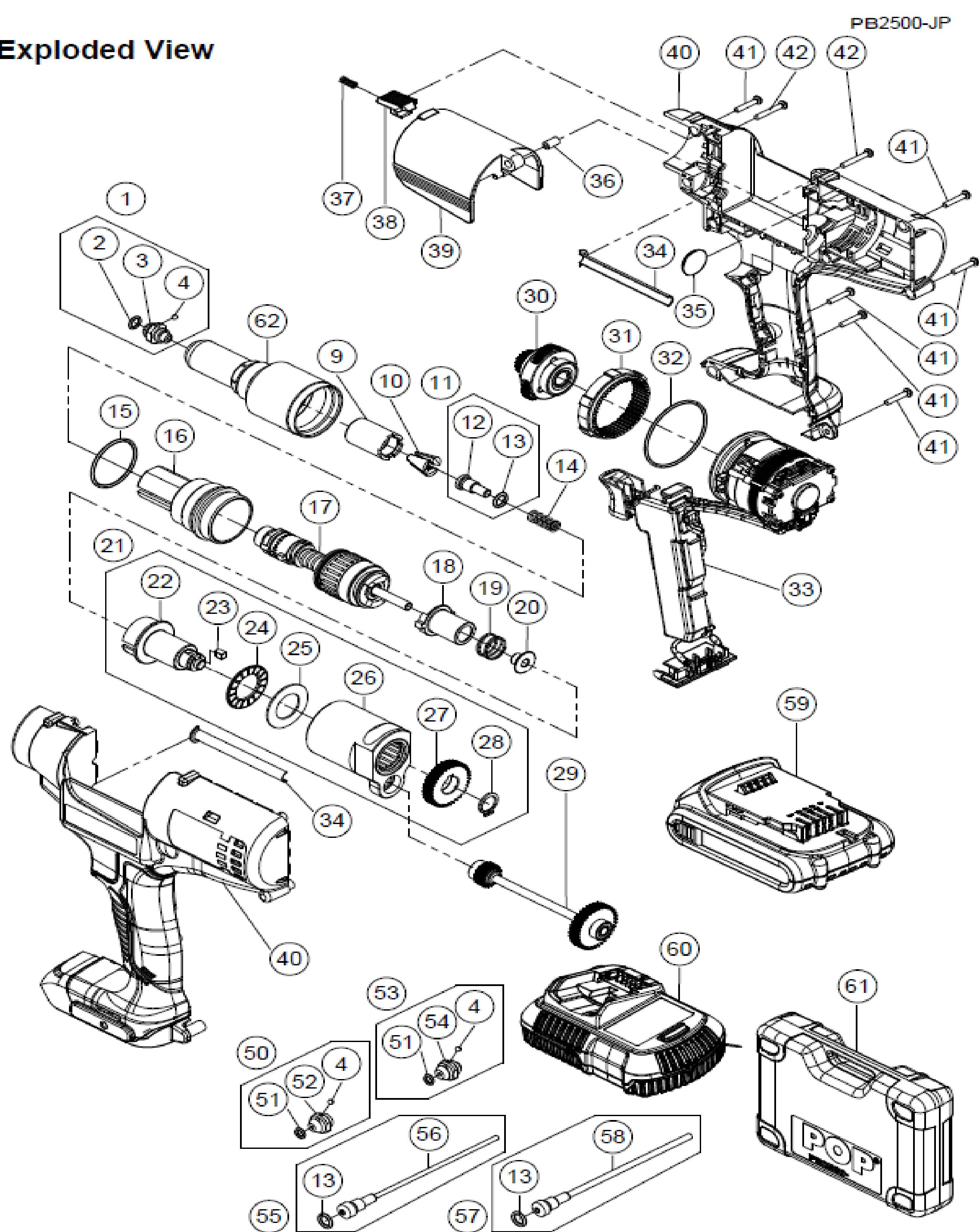
PB2500-JP,NA,GB,QW TOOL KIT
