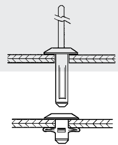
Plastic rivet before and after set.
