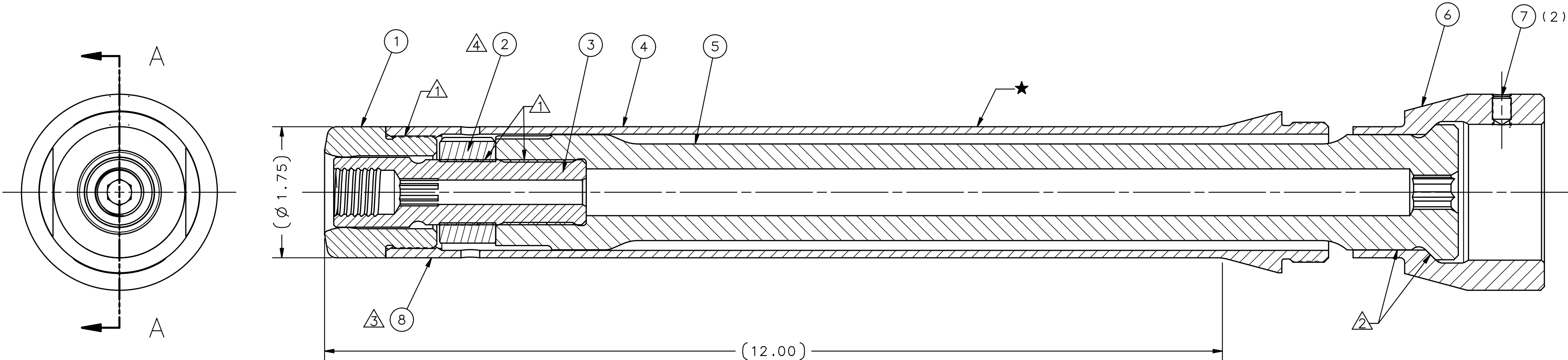
SECTION A—A
