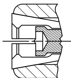
KRIMPER & STOP ASSY. IN KRIMP POSITION
