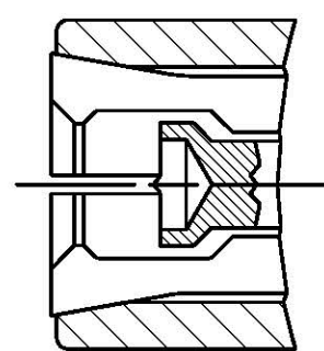
KRIMPER & STOP ASSY. IN KRIMP POSITION
