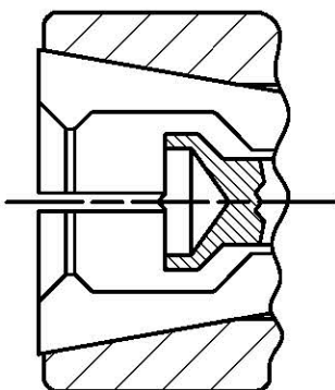
KRIMPER AND STOP ASSEMBLY SHOWN IN KRIMP POSITION
