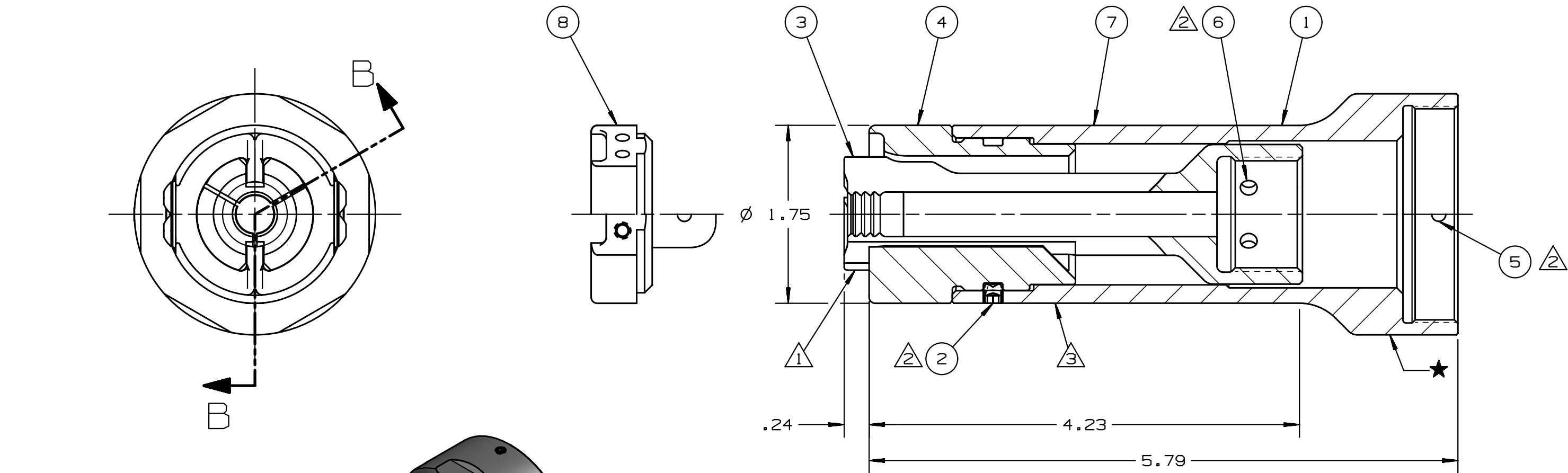
SECTION B-B
