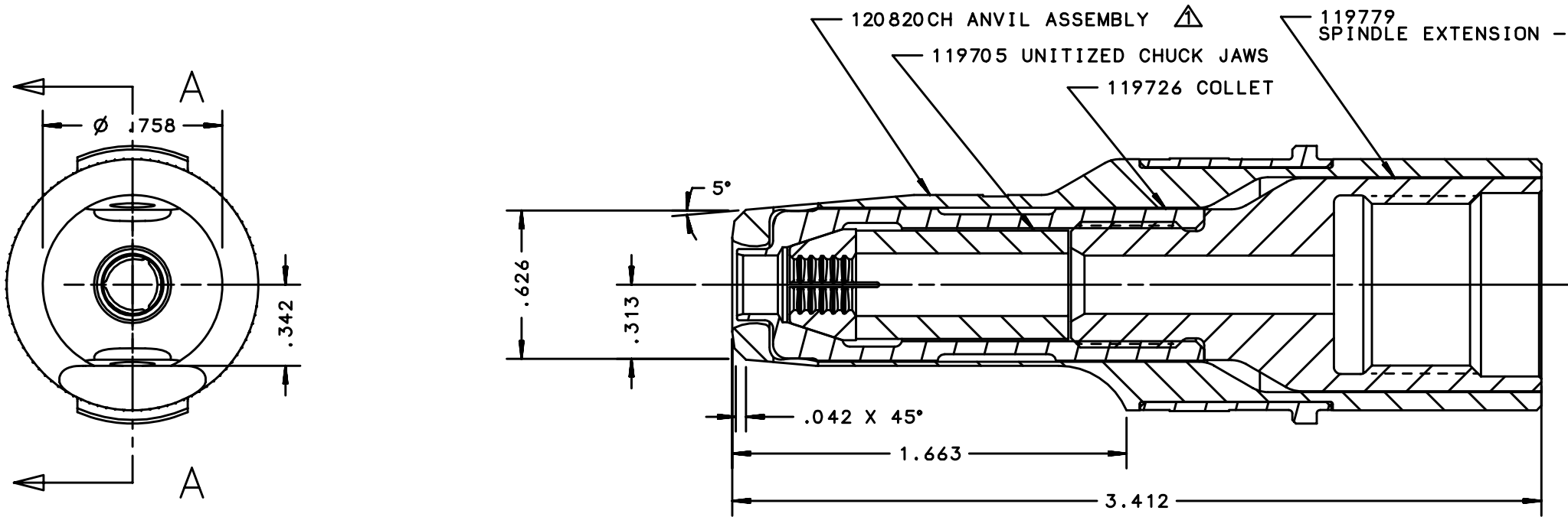
SECTION A—A
