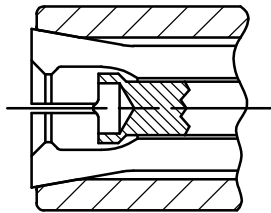
KRIMPER AND STOP ASSEMBLY SHOWN IN KRIMP POSITION
