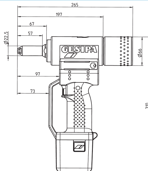
Above PowerBird® Gold Edition without pressure trigger
